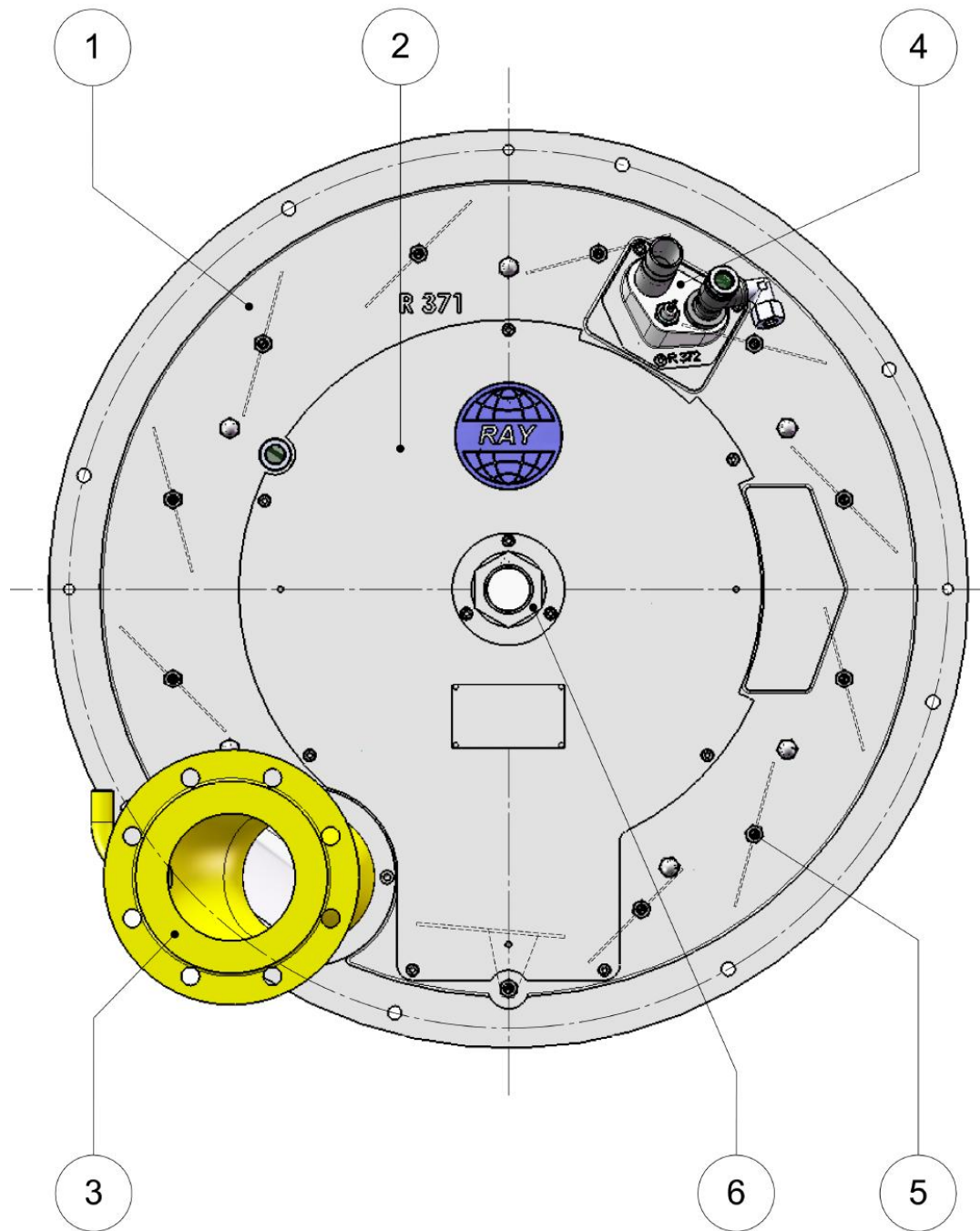
Frontansicht / Front view
